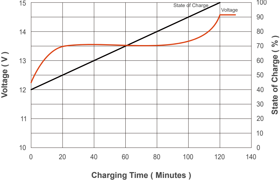
State of Charge Curve ( 0.5C, 25°C )
